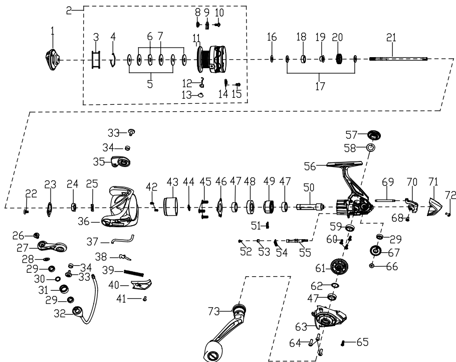
EXPLODED VIEW OF CS8-4000
